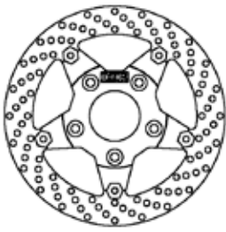
23B-HD220-01 (FH:27mm) Center hole: 50.3mm Bolt hole: 8.5mm
